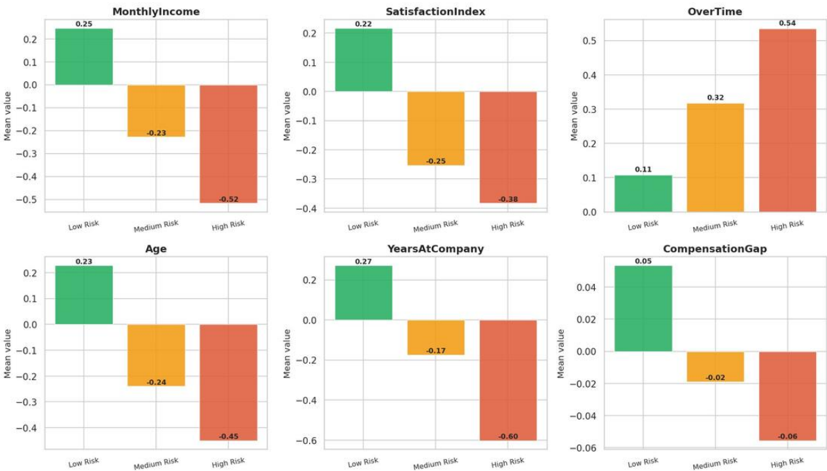
Figure 9 — Feature profiles by risk tier. All six features show clear monotonic separation across tiers.
